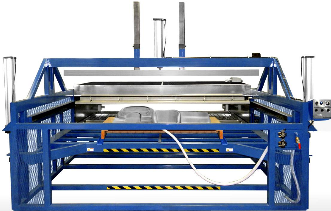
Model BV E-Class 53x103 Upper and Lower Heat Upper and Lower Tooling Table
